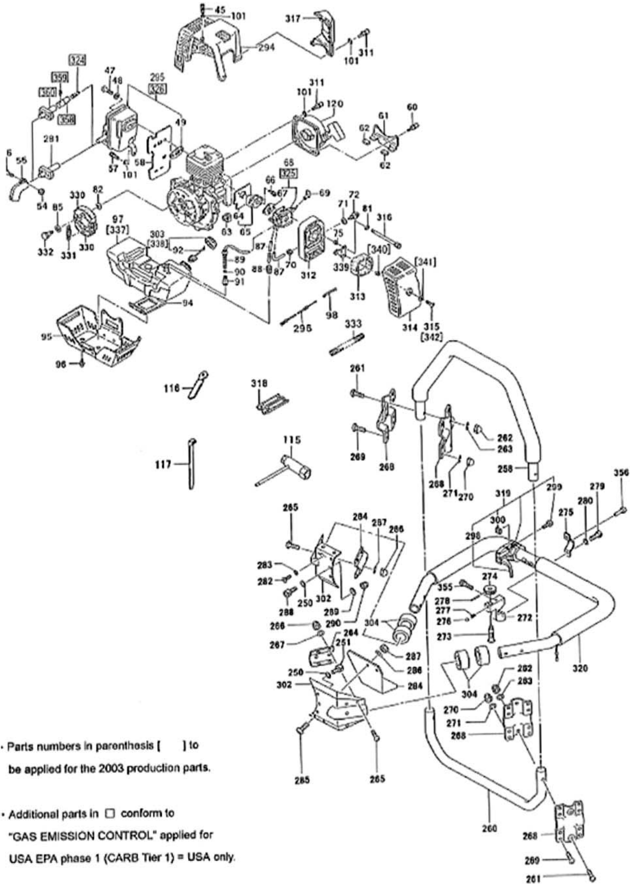
FIG.2 ENGINE COMPONENTS – EXPLODED DIAGRAM DRAWING
